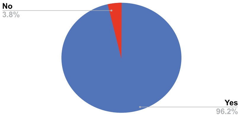
Figure 4. Survey results
